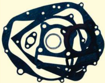
9855 004 Suzuki Yes 125
