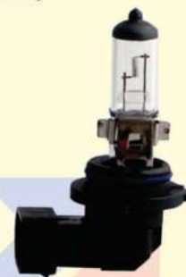
HB 4 116 4 - 12V-51W
