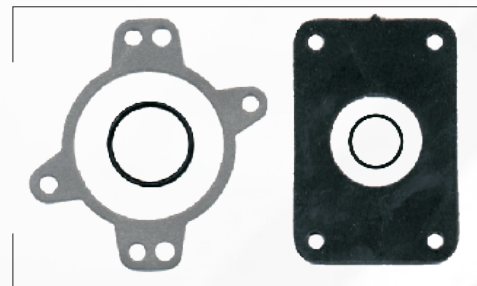
3566 570 Fiesta 1.3 Import. (Kit c/ bag.) S.Point Sist. FICEEC IV
