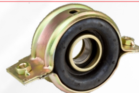
6200 800 Mancal do cardan Hilux 4x2 97...04 Hilux Pitbull 4x2 05...08
