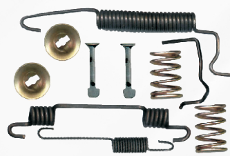
4600 193 Rep. sapata sist. varga Corsa Astra 95...96 Tigra (pino 27mm)
